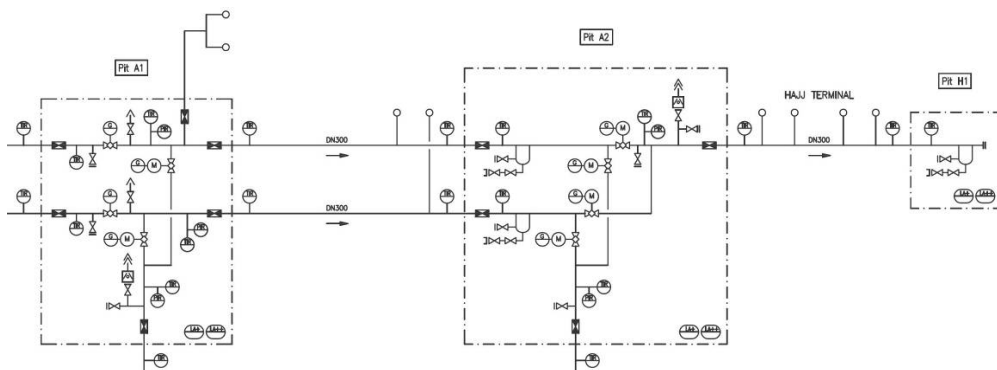
p&id aviation fuel supply, detail main feeder line
